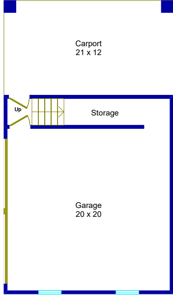
Garage First Floor
